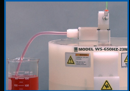
New Single Shot Pump Driven Dispenser Shown
